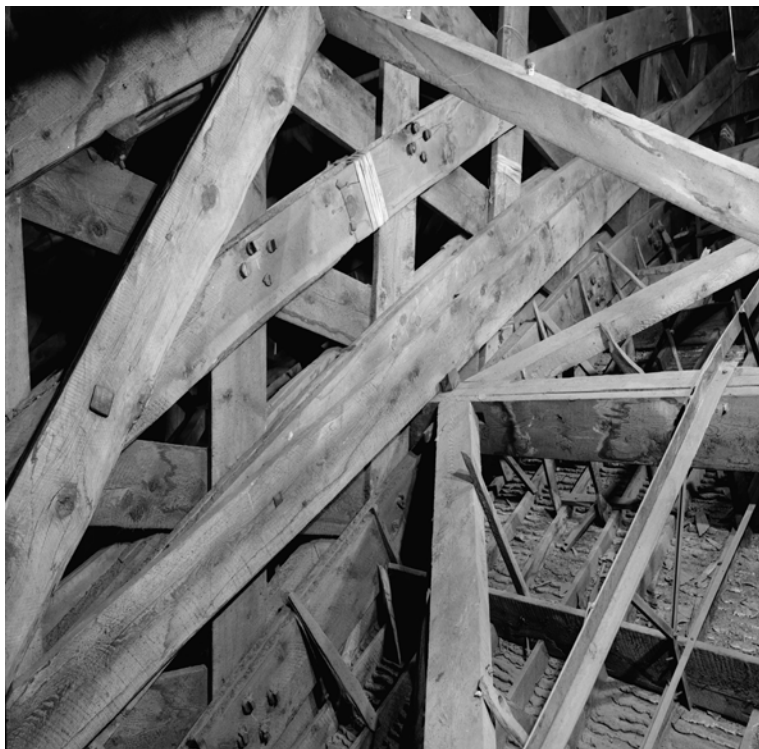
Detail of roof trusses on Salt Lake Tabernacle.
