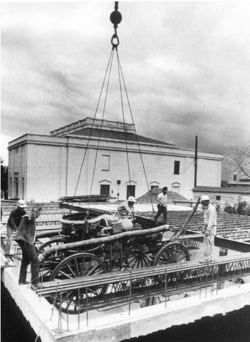
Roosevelt steam fire engine as it was lowered into Carriage House basement. (DUP Photo Collection)
